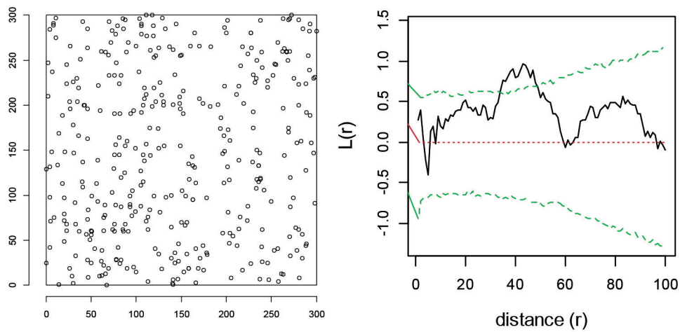
Figure 11. Indices L(r) des semis de points de (diamètre \geq 10 cm) Scorodophloeus zenkeri en 2021 dans le bloc Nord. Figure 11. L(r) indices of point seedlings of (diameter \geq 10 cm) Scorodophloeus zenkeri in 2021 in the North block.
