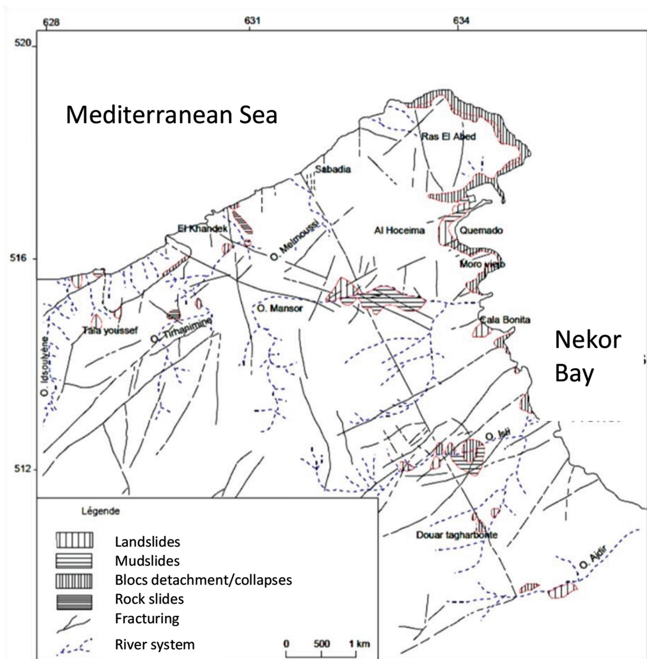
Figure 6. Map of landslides located in the study area (after Talhaoui et al. 2005).
