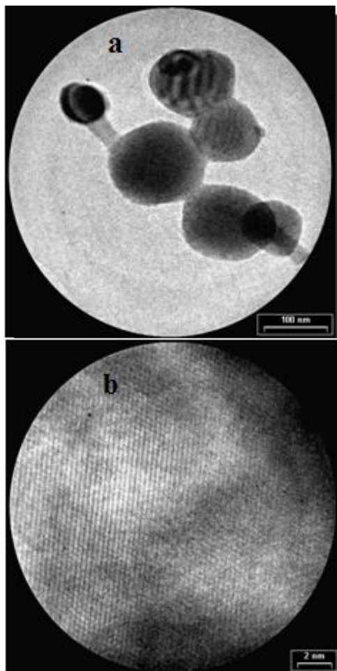
Figure 3. TEM images of the polycrystalline ZnO powder (a, b) (Bouloudenine 2006).
