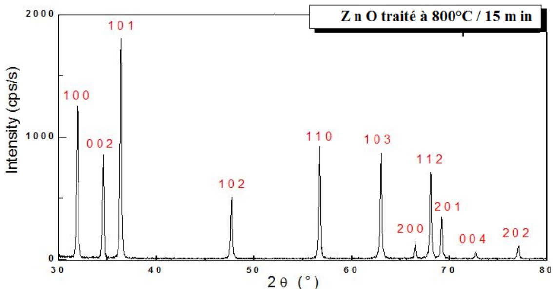
Figure 2. Ray "X" diffraction pattern of ZnO powder, CoK \alpha 1 ( \lambda=1.789\text{\AA} ) (Bouloudenine 2006).
