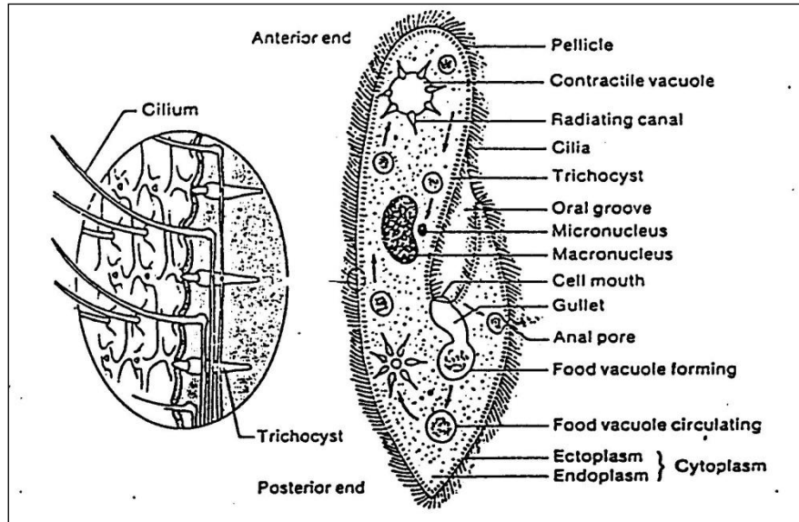
Figure 1. General appearance of a paramecium (Beaumont & Cassier 1998).
