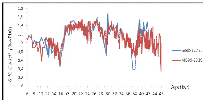
Figure 3. Correlation between the benthic \delta^{13}\text{C} records of Geob 12723 and the core MD99-2339.
