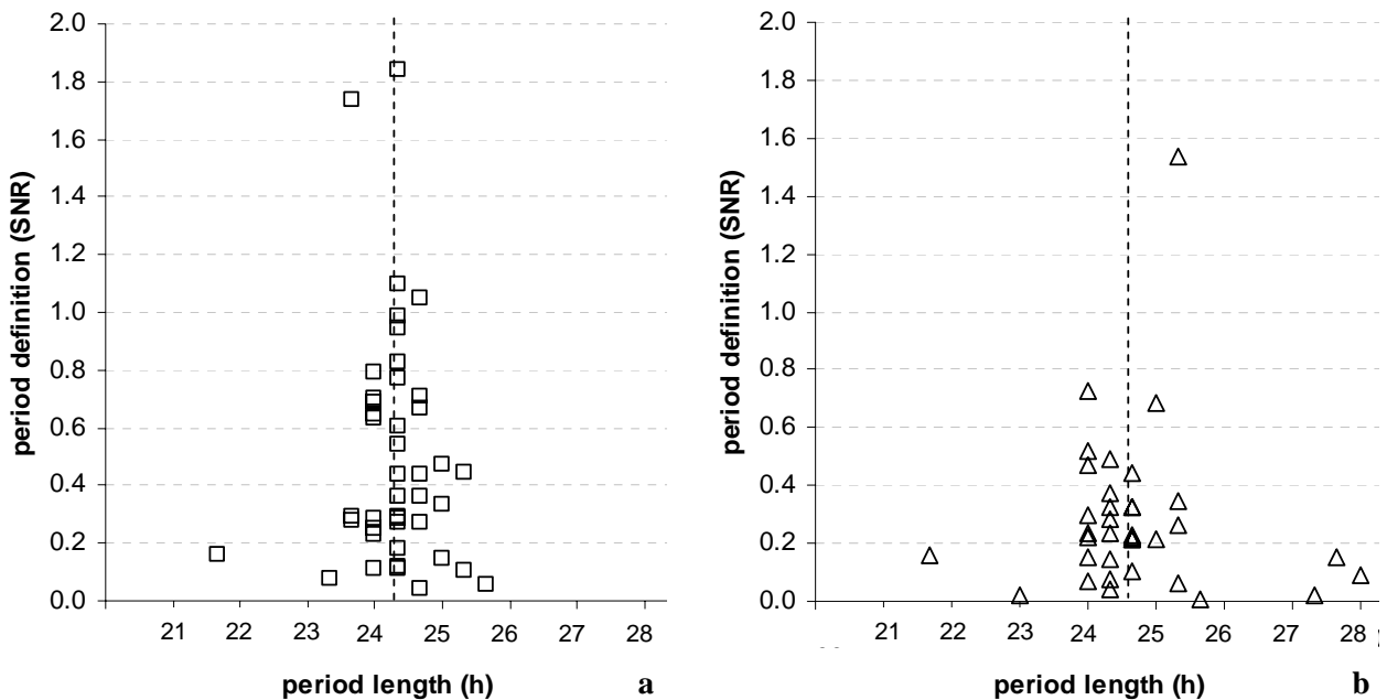
Figure 1: Scatter plots of the period definition: a) Talitrus saltator ; squares, individual means; b) Orchestia gammarellus ; triangles, individual means. The mean period length is represented as a dotted line.
